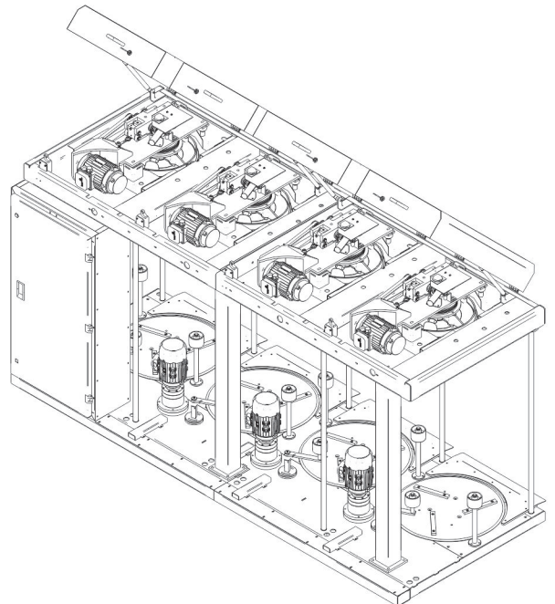
Four Head with individual drive on Quad coiler
