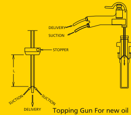
Topping Gun For new oil
